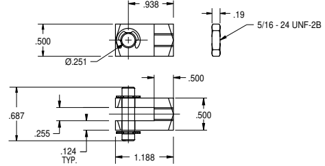
B-127004 1-1/16" Bore
