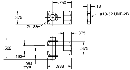
B-127004 1-1/16" Bore
