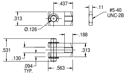
B-127001 5/16" Bore
