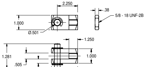
B-127007 3" Bore
