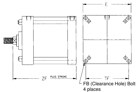
Mount Code E4 NFPA ME4
