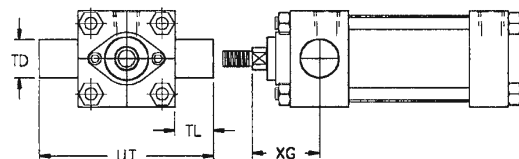
Mount Code T6 (Removable Aluminum Trunnion Ears)
