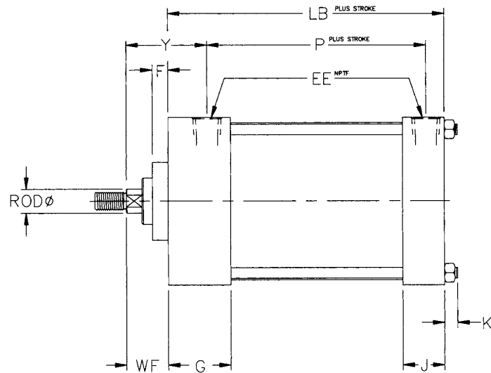
Mount Code X0 NFPA MX0
