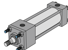
X3 Mount Extended Tie Rods - Head End
