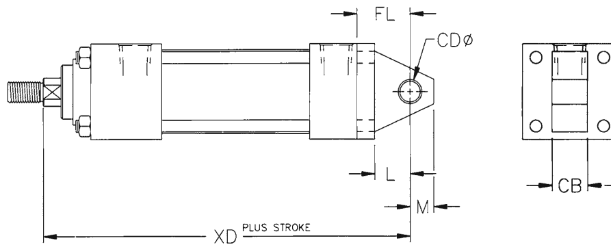
Mount Code P4 NFPA MP4
