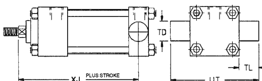
Mount Code T7 (Removable Aluminum Trunnion Ears)
