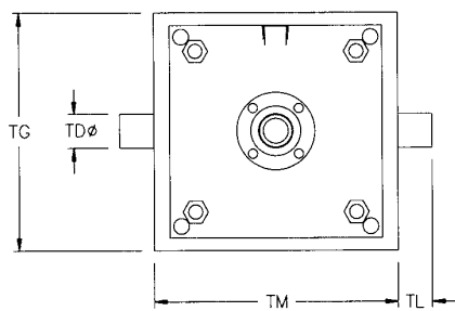
Mount Code T4
