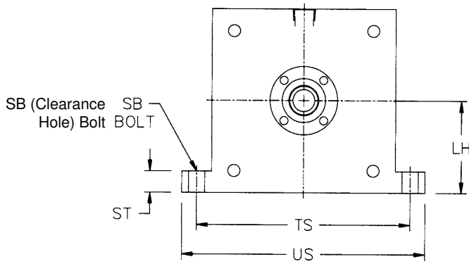
Mount Code S2
