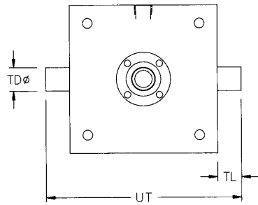
Mount Code T1
