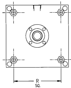
Mount Code X3
