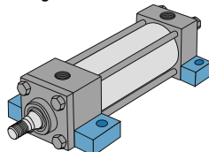
S2 Mount Side Lugs
