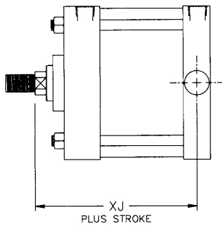
Mount Code T2
