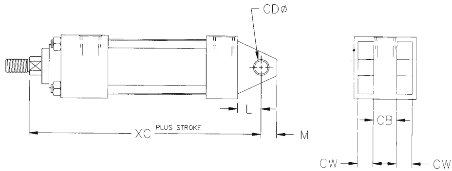
Mount Code P1 NFPA MP1
