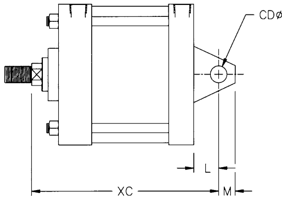
Mount Code P1
