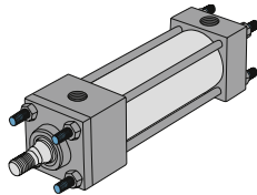
X1 Mount Extended Tie Rods - Both Ends
