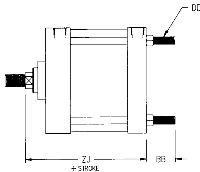
Mount Code X2
