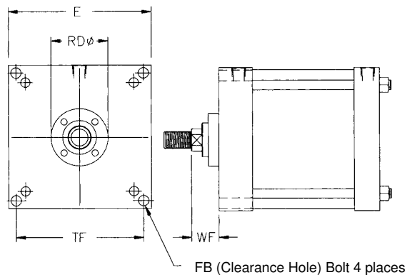
Mount Code X0 NFPA MX0
