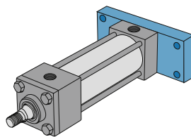
F2 Mount Cap Rectangular Flange
