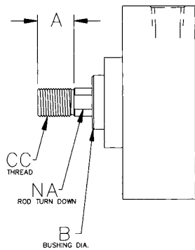
Style #2 (Optional Male)
