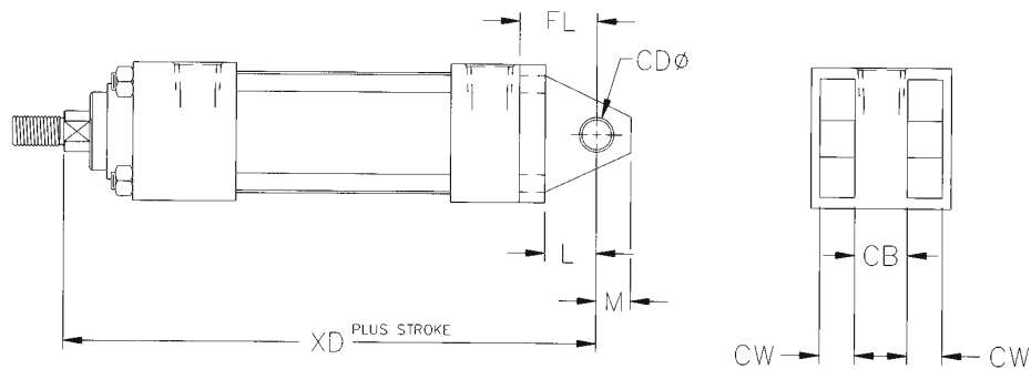
Mount Code P2 NFPA MP2
