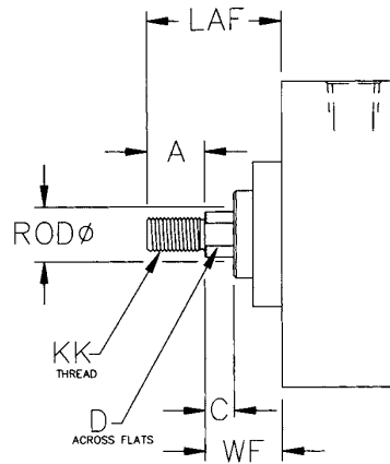
Style #1 (Standard Male)
