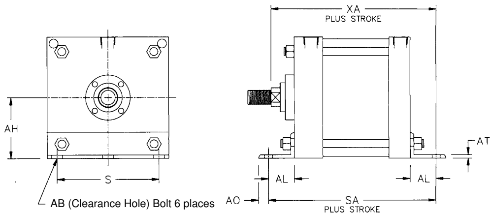
Mount Code S1
