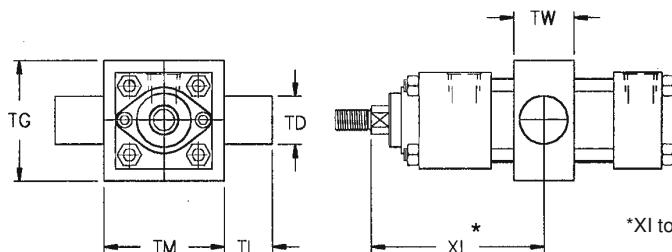
Mount Code T8 (Removable Trunnion Ears)
