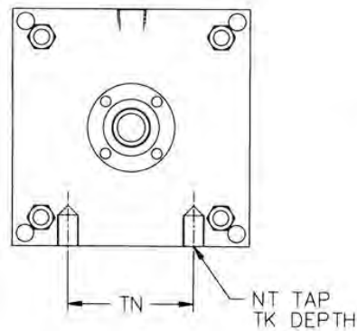
Mount Code S4
